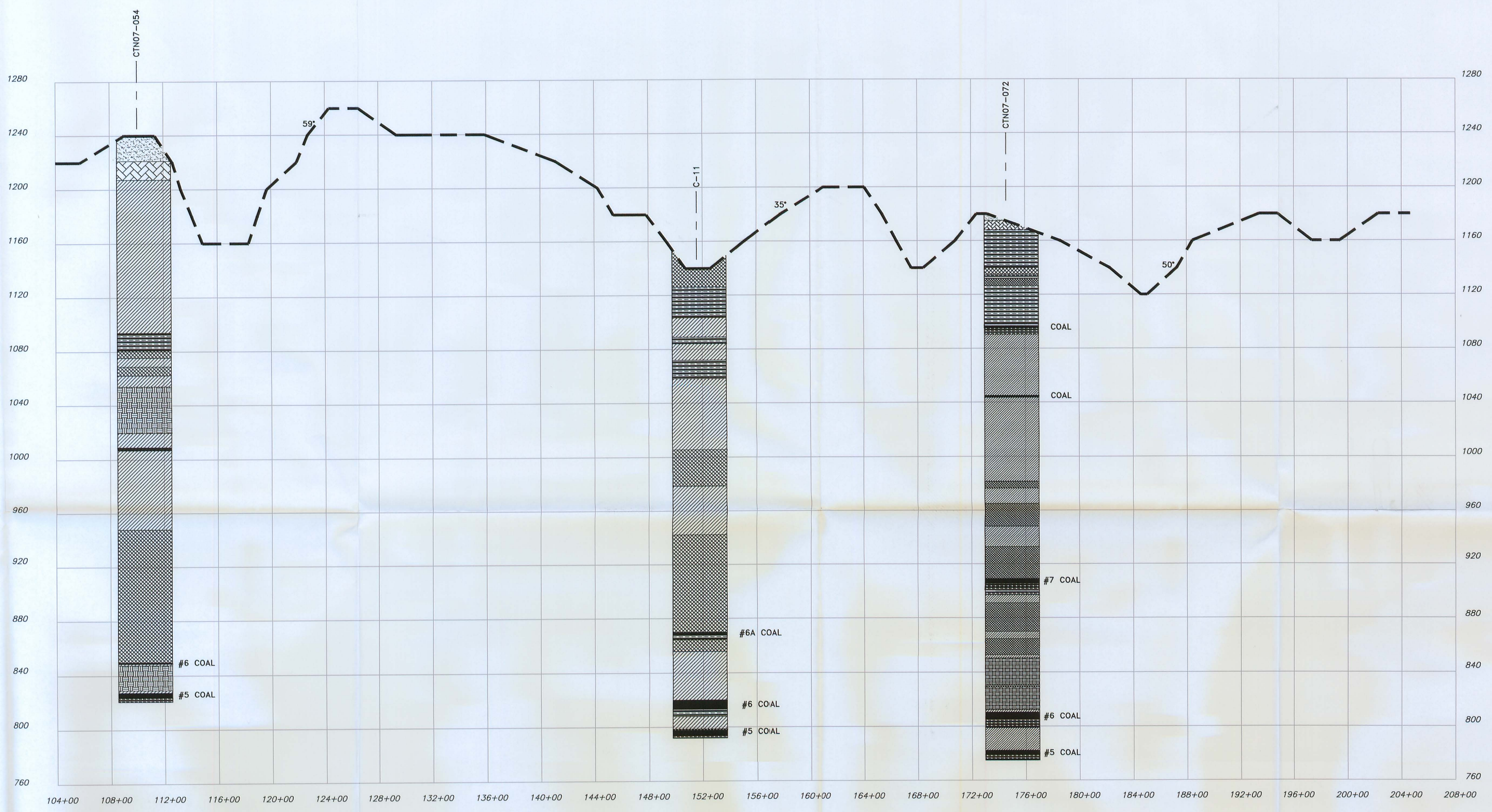
CROSS SECTION B-B HORIZONTAL SCALE: 1"=400' VERTICAL SCALE: 1"=40' STATION 104+00 TO 208+00
